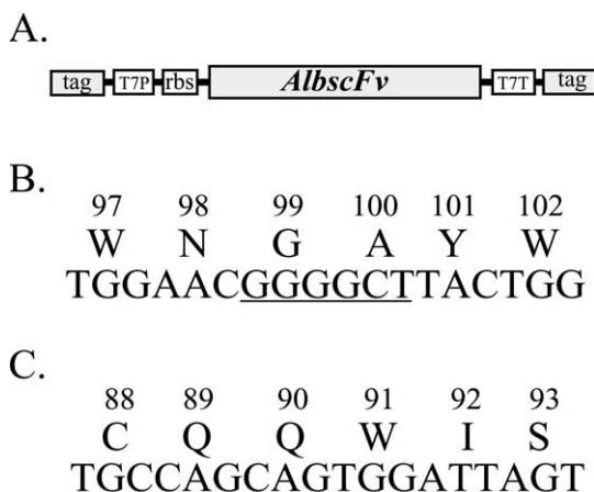
Fig. 2. Design of the DNA templates for experiments. A: Schematic representation of the DNA template ready for amplification by PCR and in vitro coupled transcription/translation. It contains a DNA tag (tag) serving as primer annealing sites at both ends, T7 promoter (T7P), ribosome binding site (RBS), anti-HSA-scFv encoding gene ( AlbscFv ), and T7 terminator (T7T). B: The sequence at the mutation site (underline) in the V_H of the DNA templates that were used in the investigation of equality of amplification in the multiplex-PCR. C: The sequence at the mutation site (underline) in the V_L of the library anti-HSA-scFv(QW).
